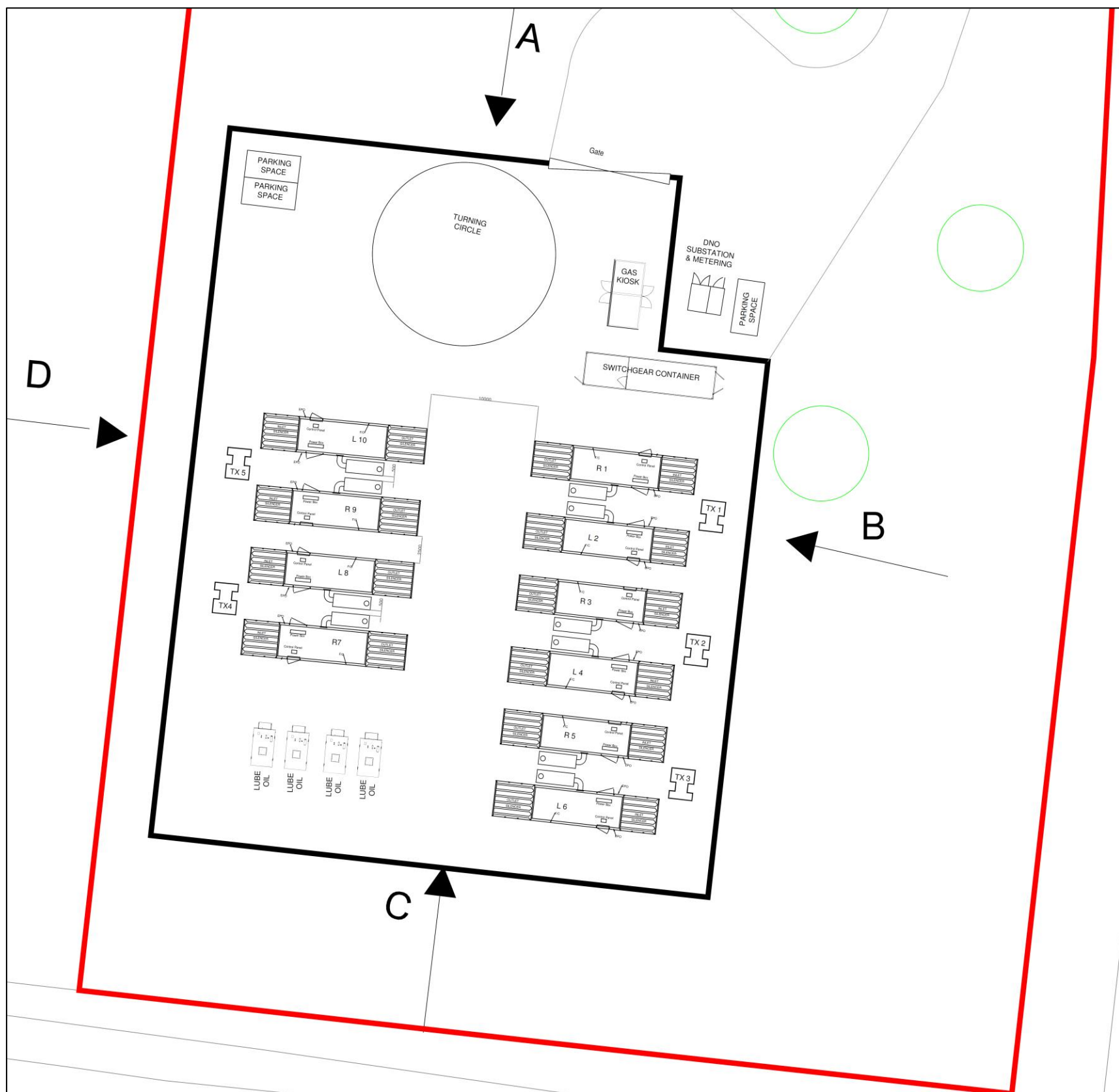
Figure B1 Plant Compound Layout
