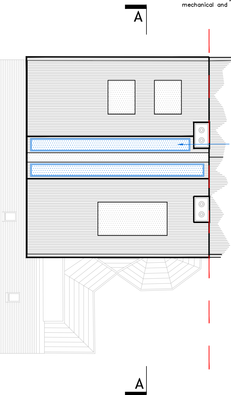
ROOF PLAN 1:100
