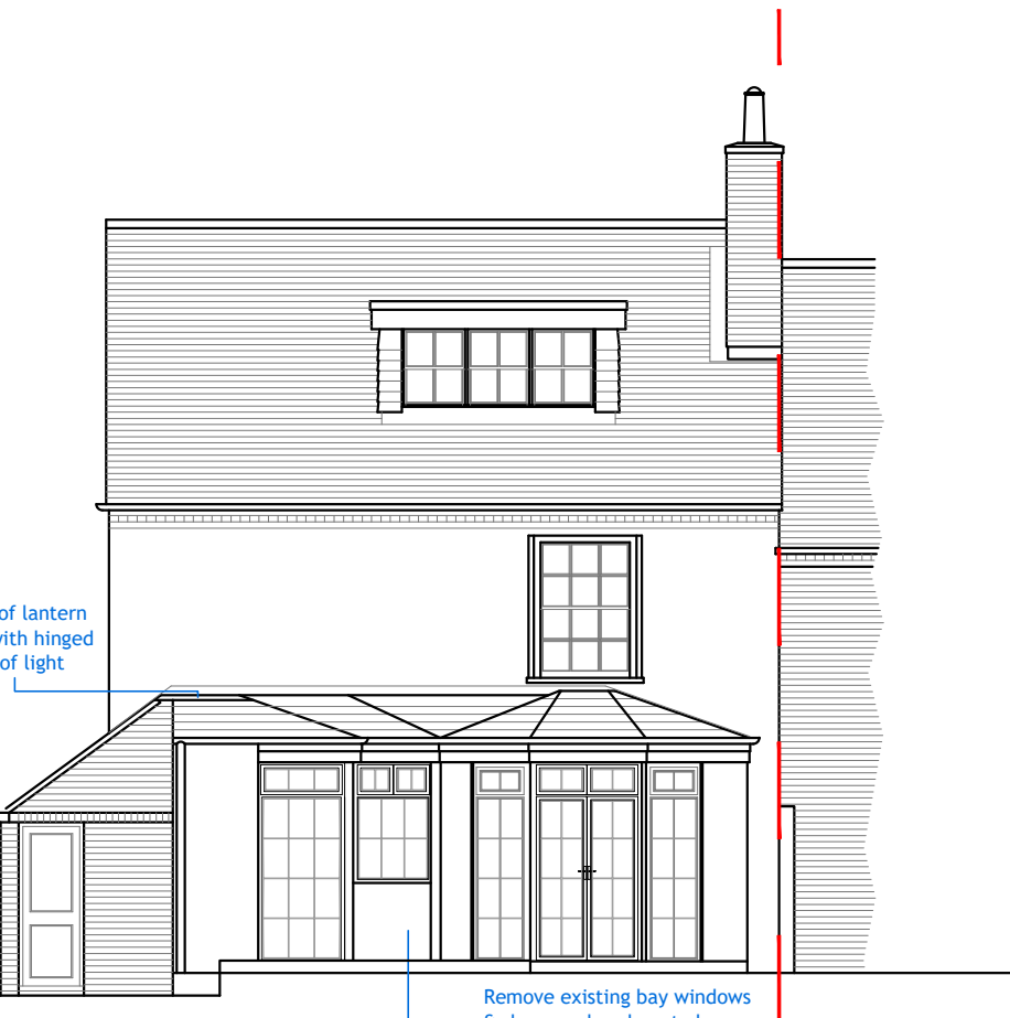
SIDE ELEVATION 1:100
