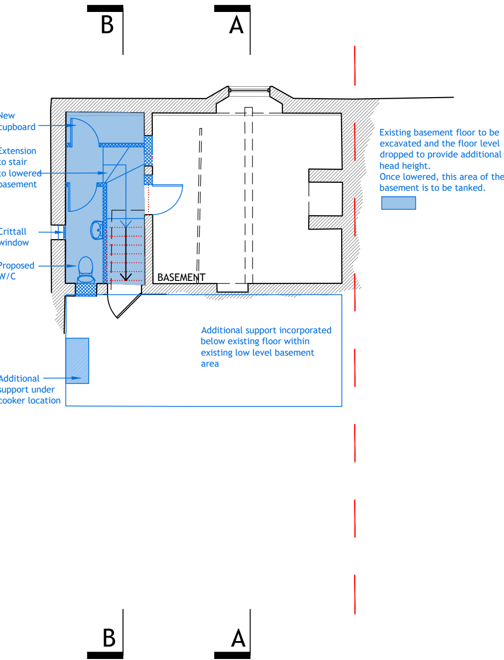
BASEMENT PLAN 1:100
