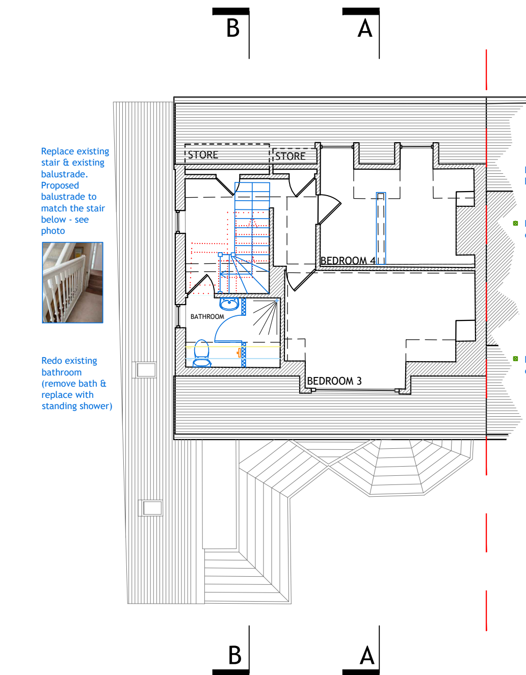
SECOND FLOOR PLAN 1:100
