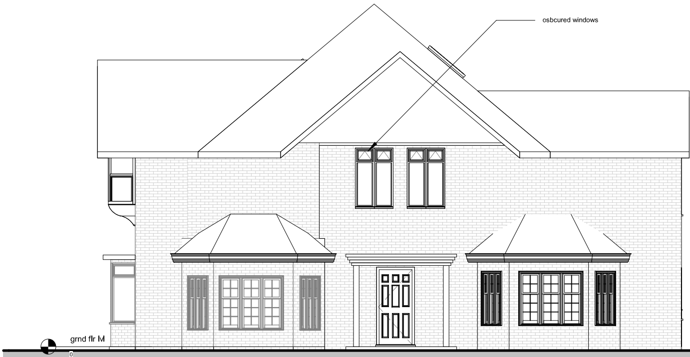
Proposed Elevation-Front
