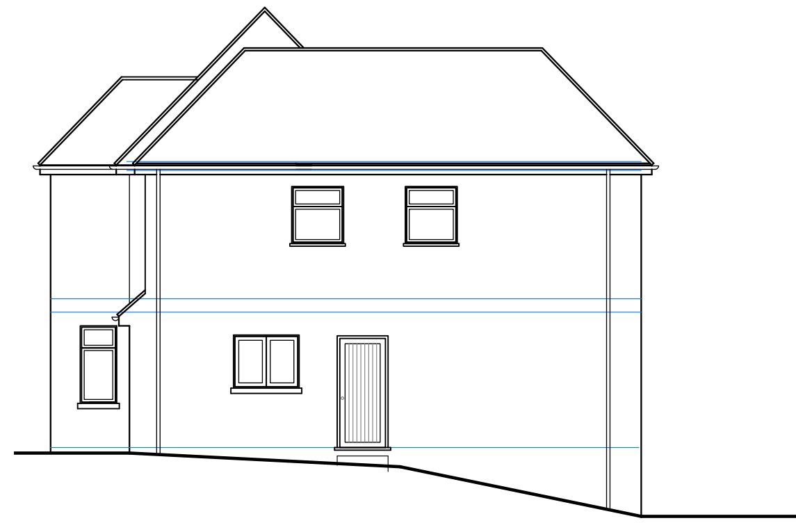
10 Proposed East Elevation Scale: 1:100
