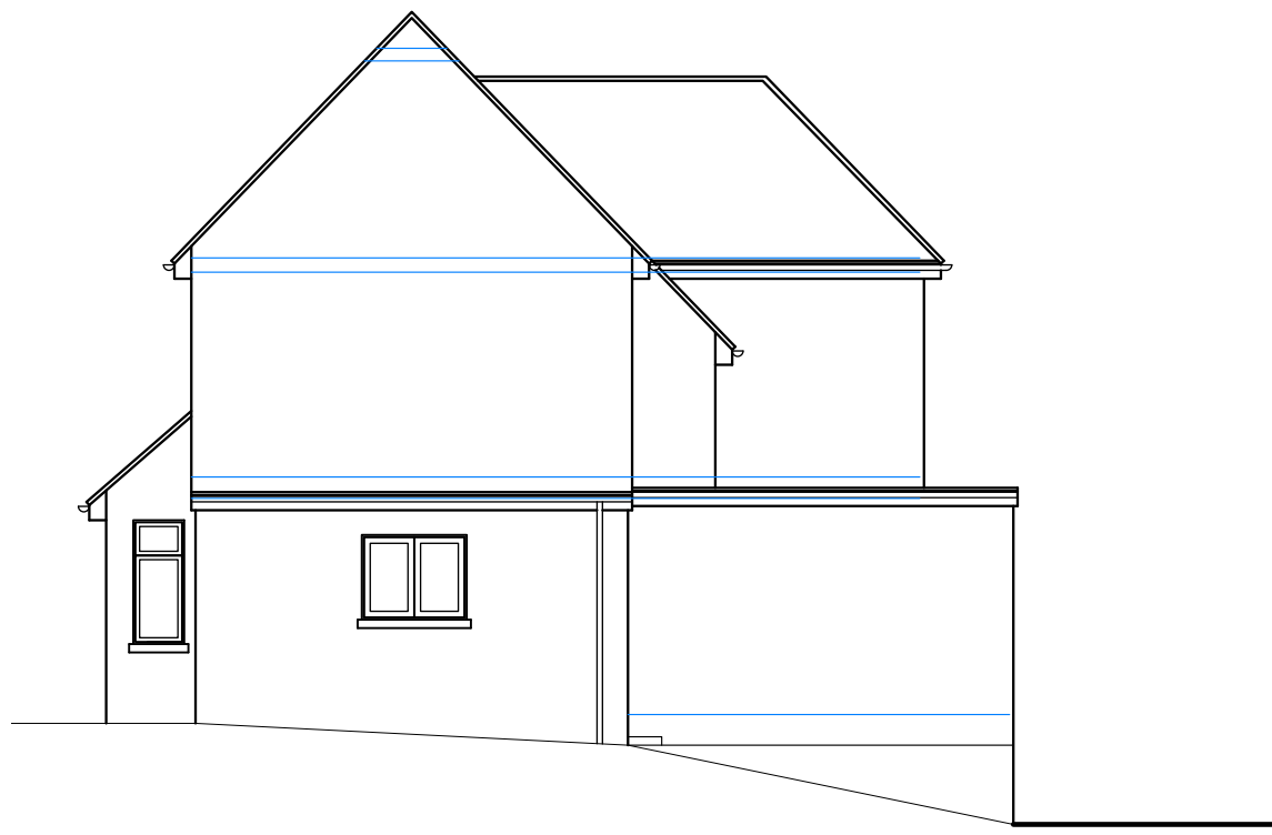
4 Existing East Elevation Scale: 1:100
