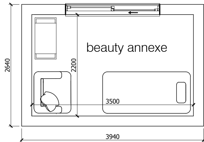
proposed annexe floor plan
