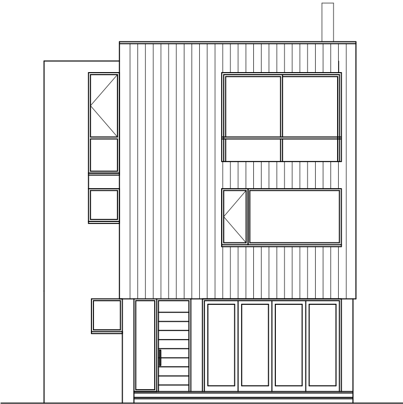
South Elevation (rear) - As Approved
