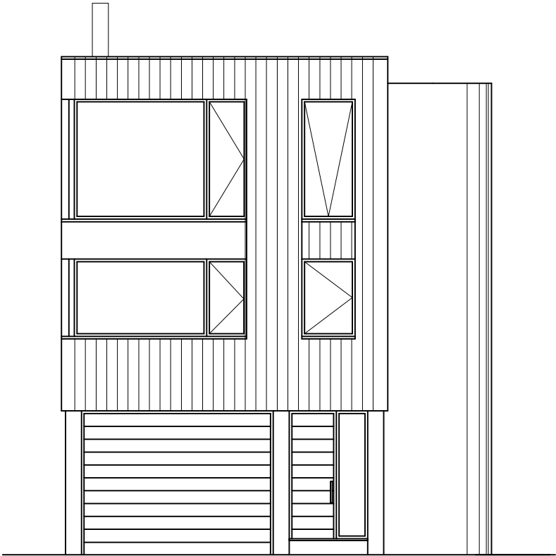
North Elevation (front) - As Approved
