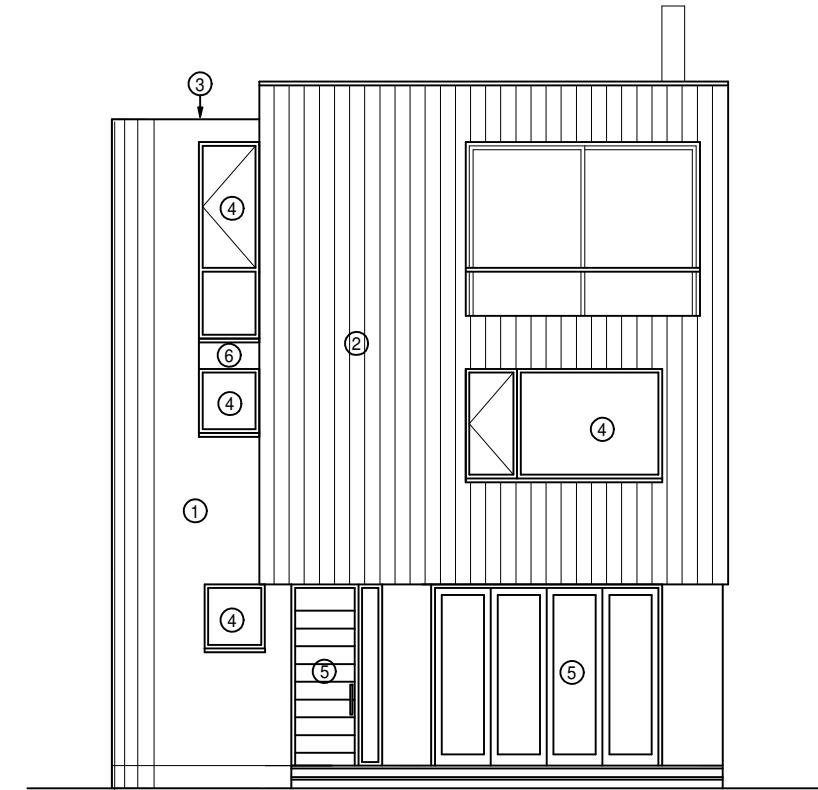
South Elevation (rear) - As Proposed
