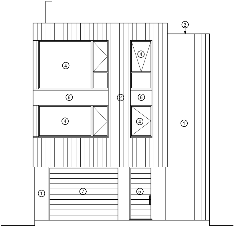
North Elevation (front) - As Proposed
