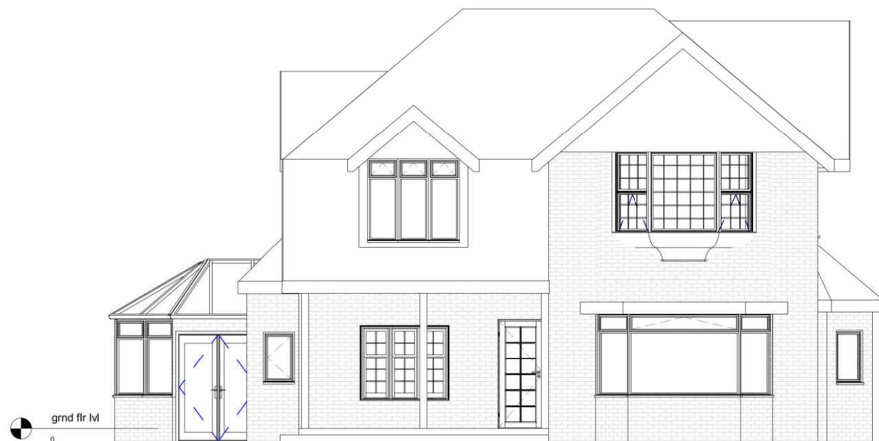
Existing Elevation-Left side
