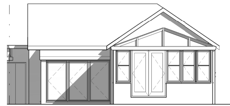
4 Existing Rear 1 : 100
