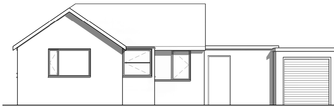
2 Existing Front 1 : 100
