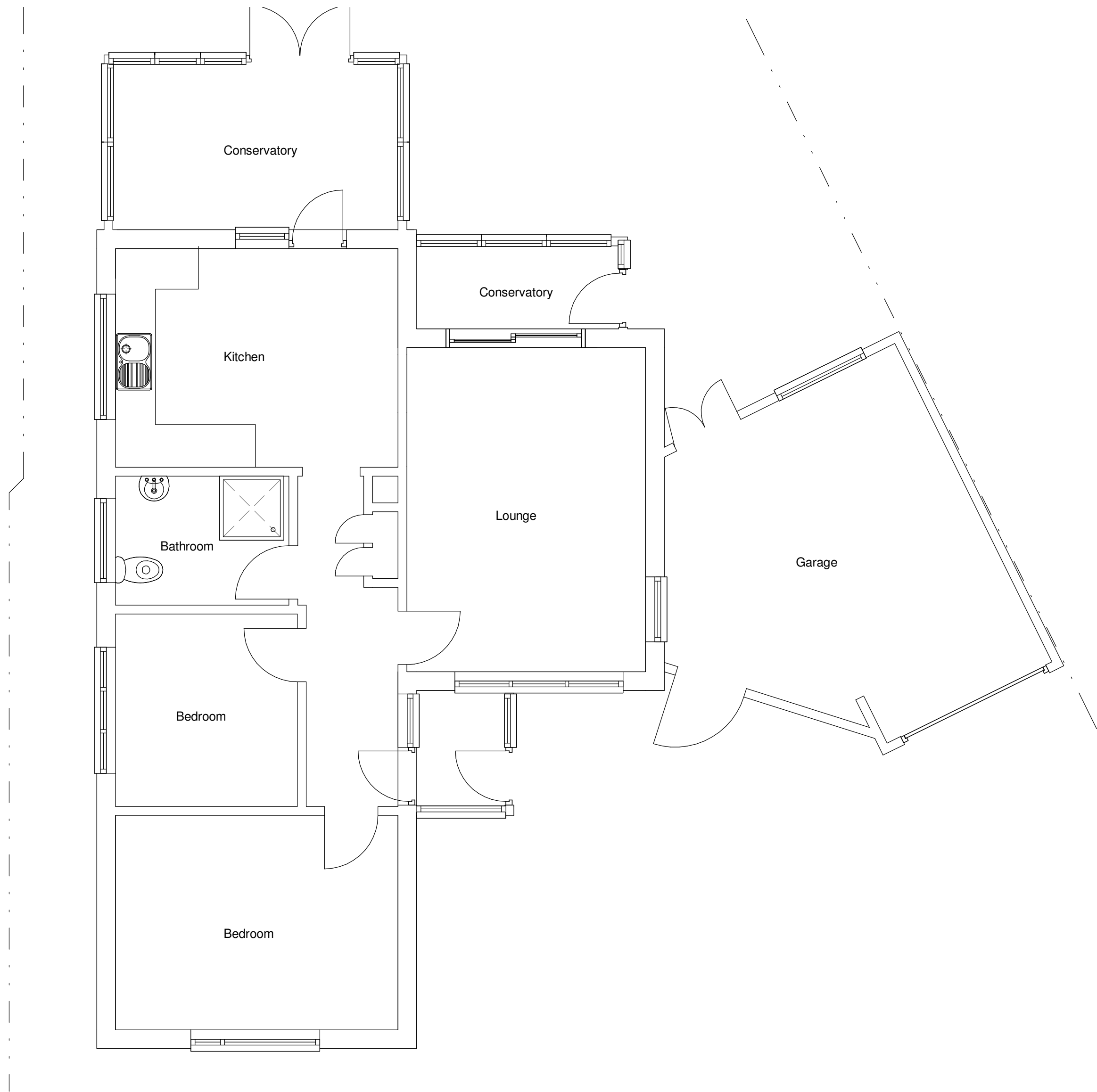
1 Existing Ground Floor 1 : 50
