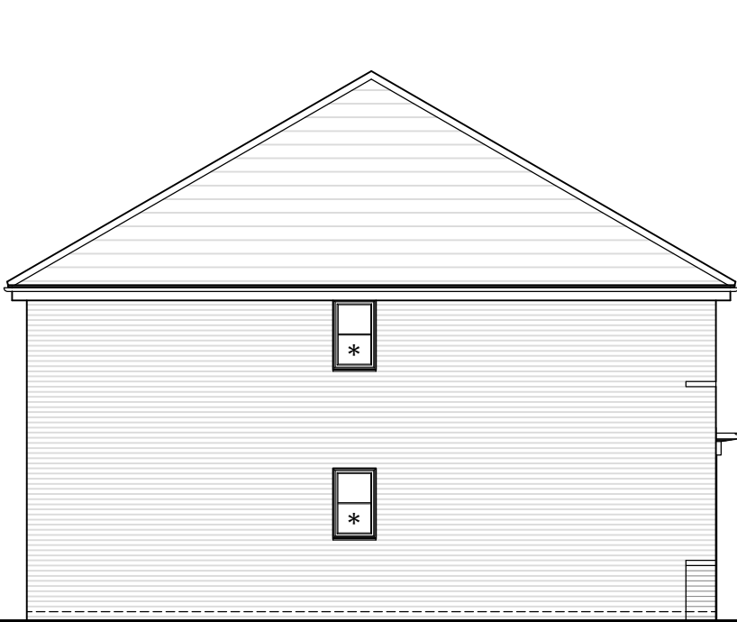
Side Elevation *No side windows to plots 137, 138, 147, 148, 149, 150, 153
