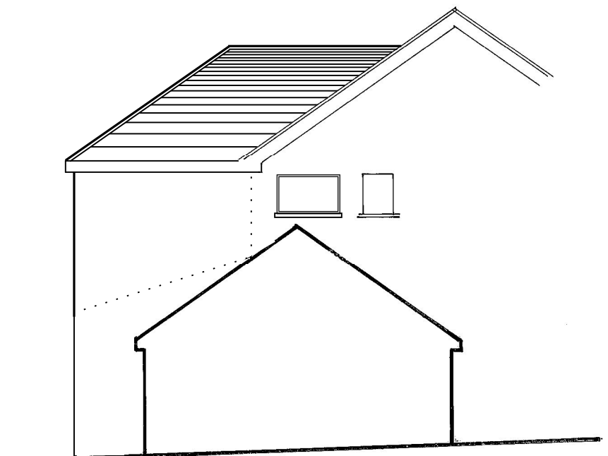
Proposed North/Side Elevation
