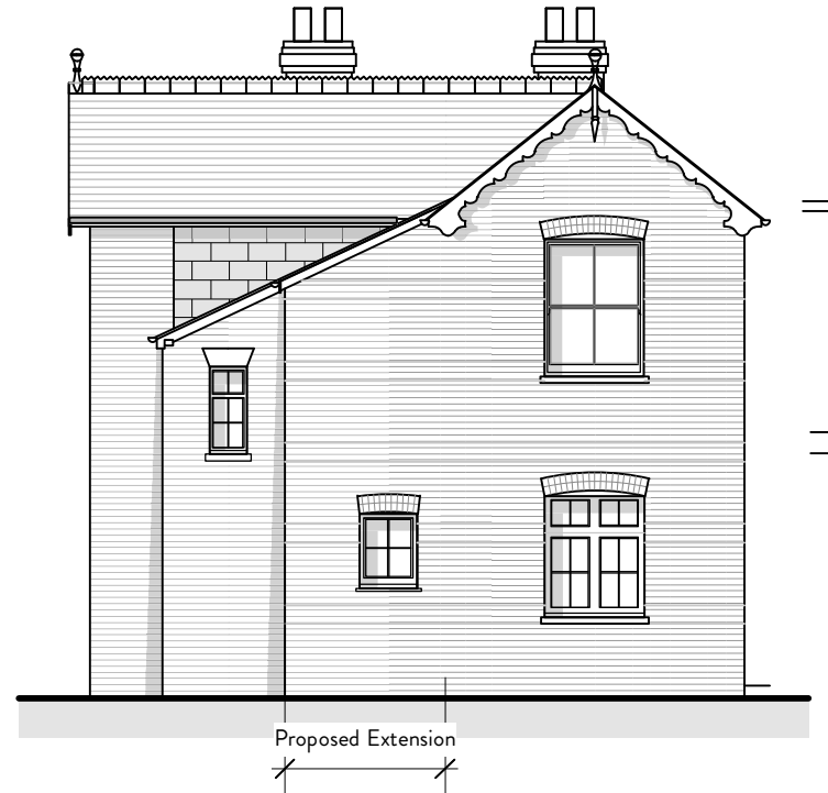
North Elevation
