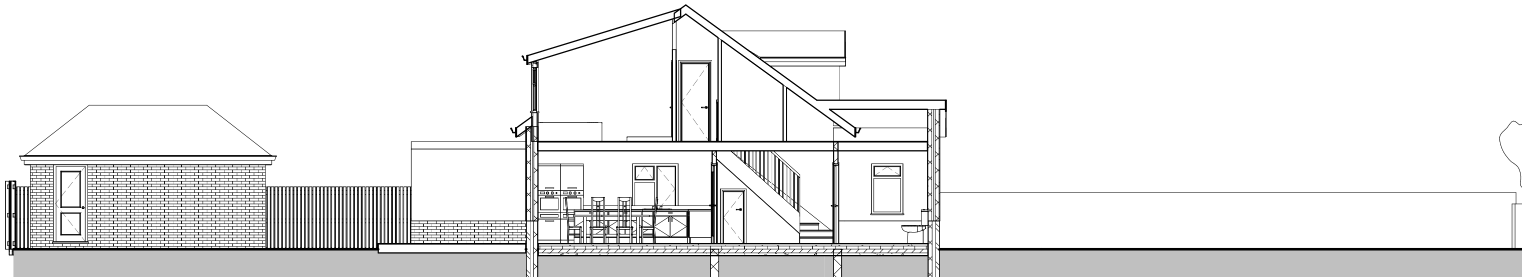
1 East West Site Section (A3) 1 : 100
