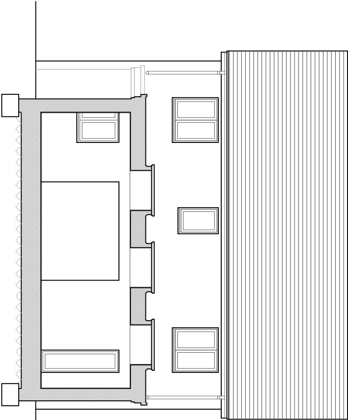
Cross-Section AA
