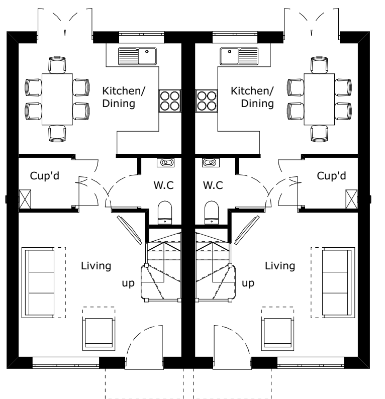
GROUND FLOOR - 1:100
