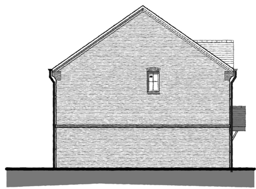
SIDE ELEVATION [1] - 1:100
