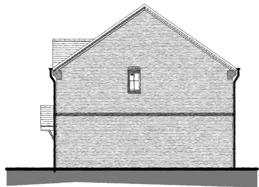
SIDE ELEVATION [2] - 1:100
