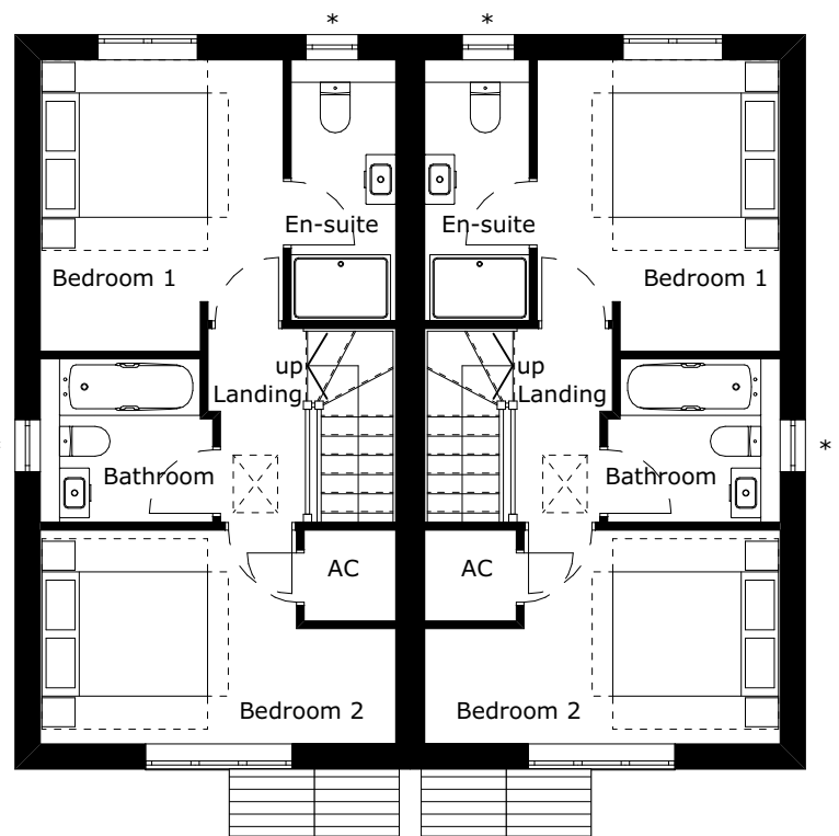
FIRST FLOOR - 1:100
