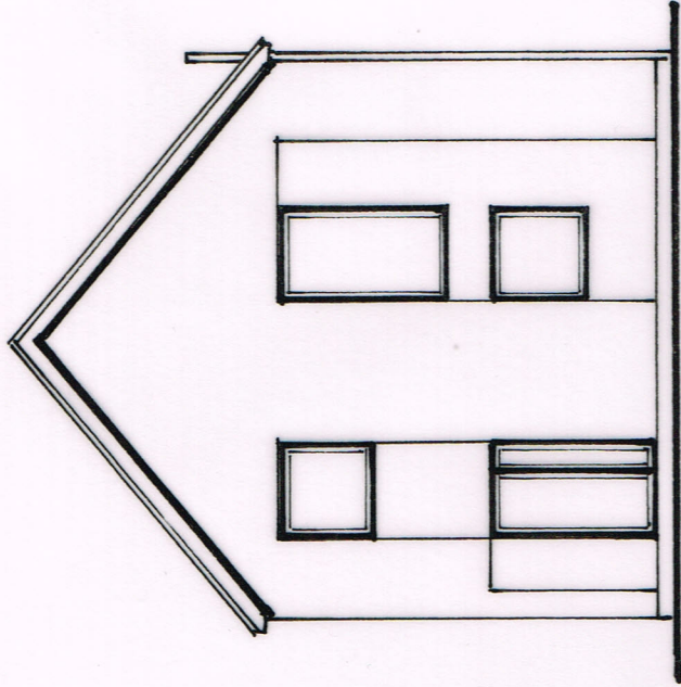
EAST ELEVATION
