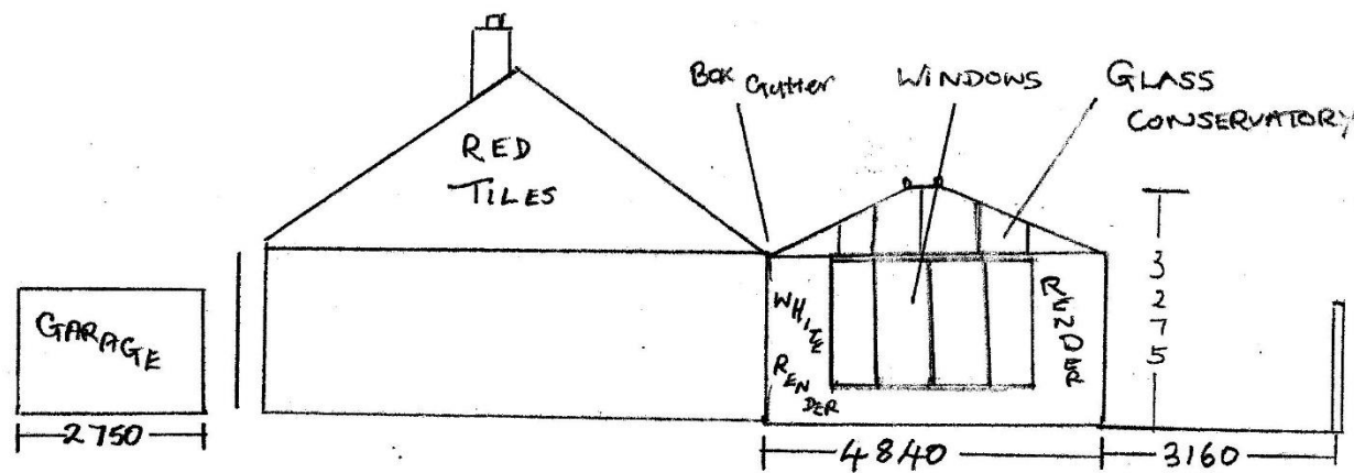
SIDE ELEVATION (NORTH) PROPOSED ELEVATION
