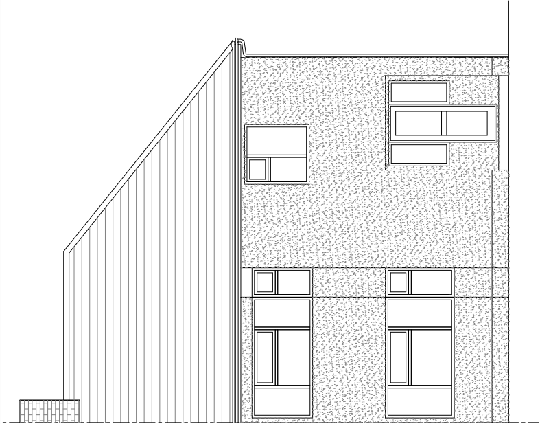
Proposed Front Elevation (No changes)
