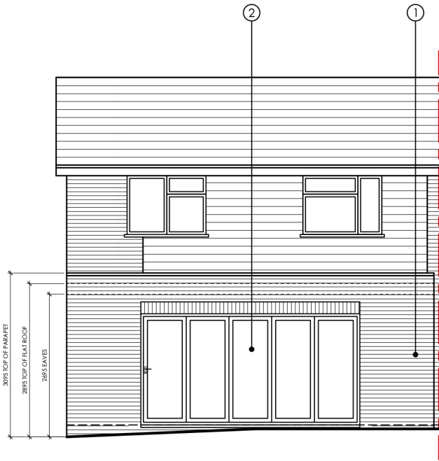
PROPOSED WEST ELEVATION
