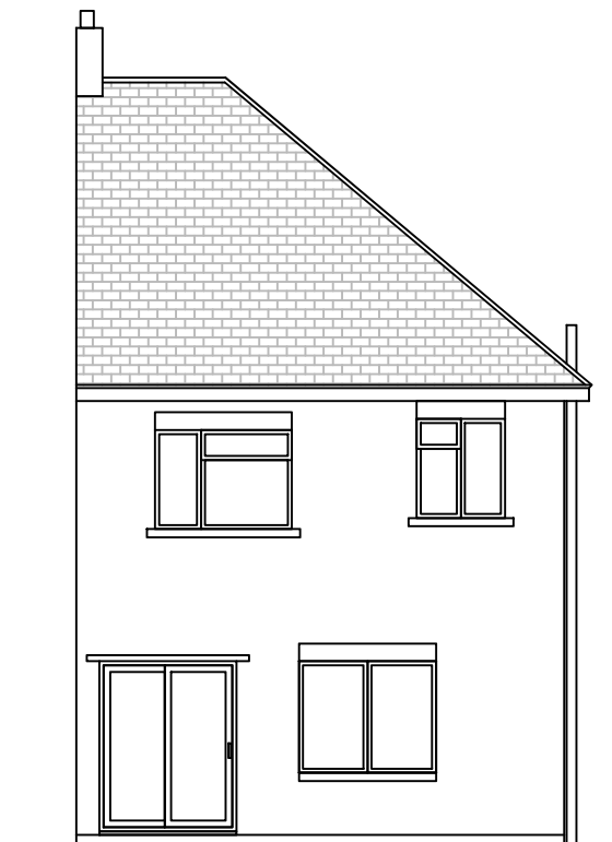
Rear Elevation
