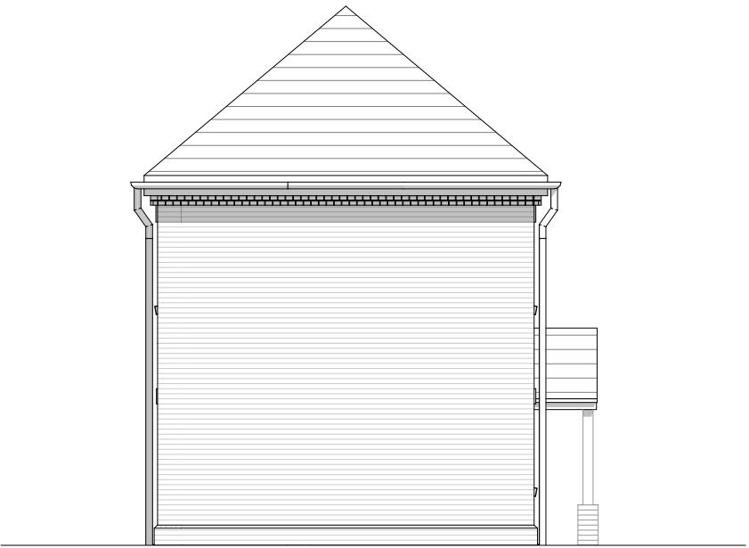
Side 2 Elevation
