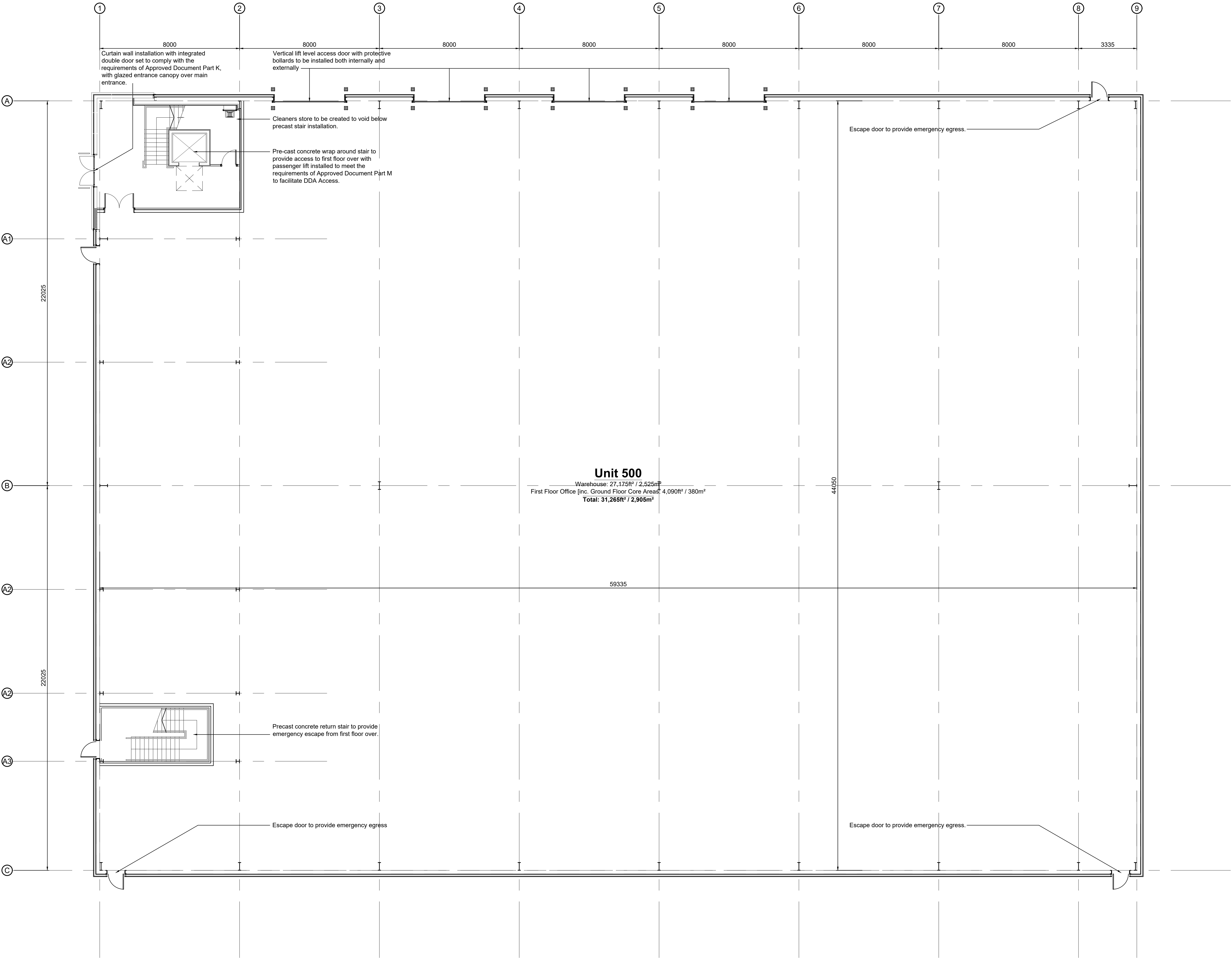
Unit 500, Building Plan_SCALE 1:100 @ A1
