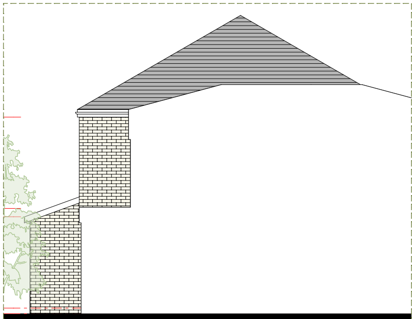
Proposed Neighbour Elevation Scale 1:100
