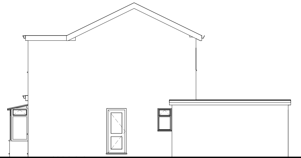
4 West Elevation 1 : 100
