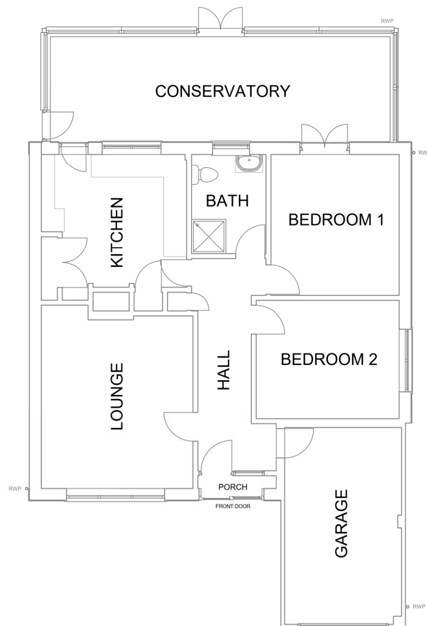
GROUND FLOOR 1 : 100
