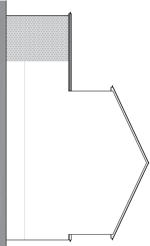
Proposed Side Elevation 1 : 100 @ A3
