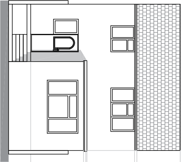
Existing Rear Elevation 1 : 100 @ A3
