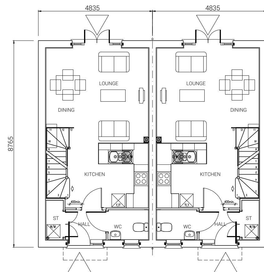
PLOT 20 GROUND FLOOR PLAN
