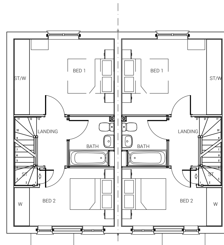
PLOT 20 FIRST FLOOR PLAN
