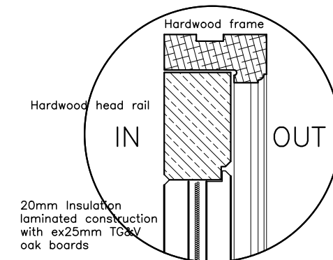
Head
