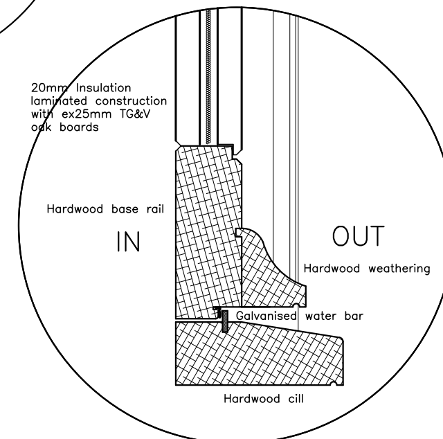
Cill/Base Rail
