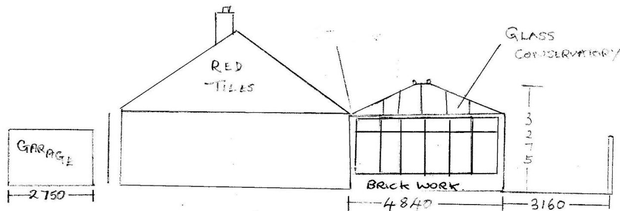
Side Elevation (North Exisiting)
