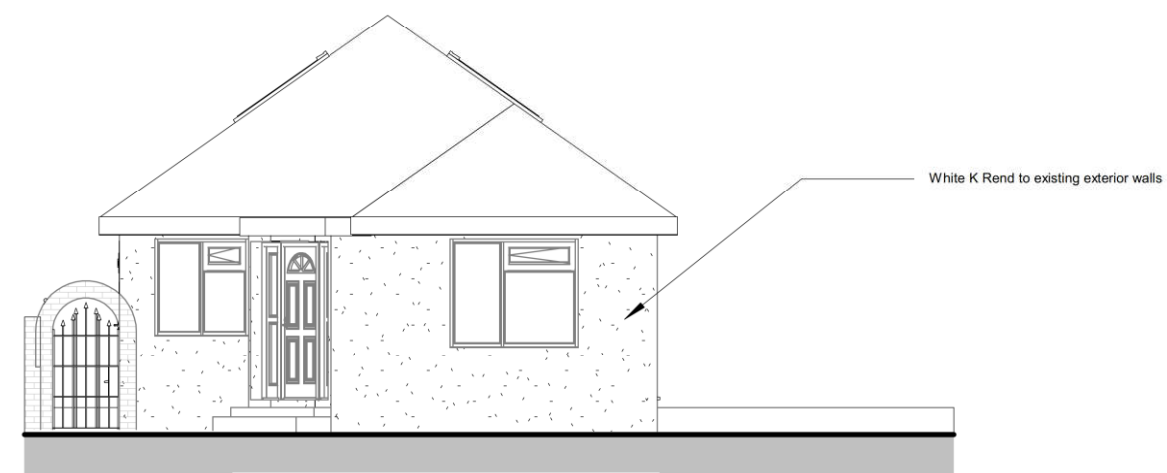
Proposed Elevation-Front
