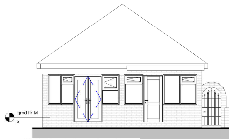
Existing Elevation-Rear
