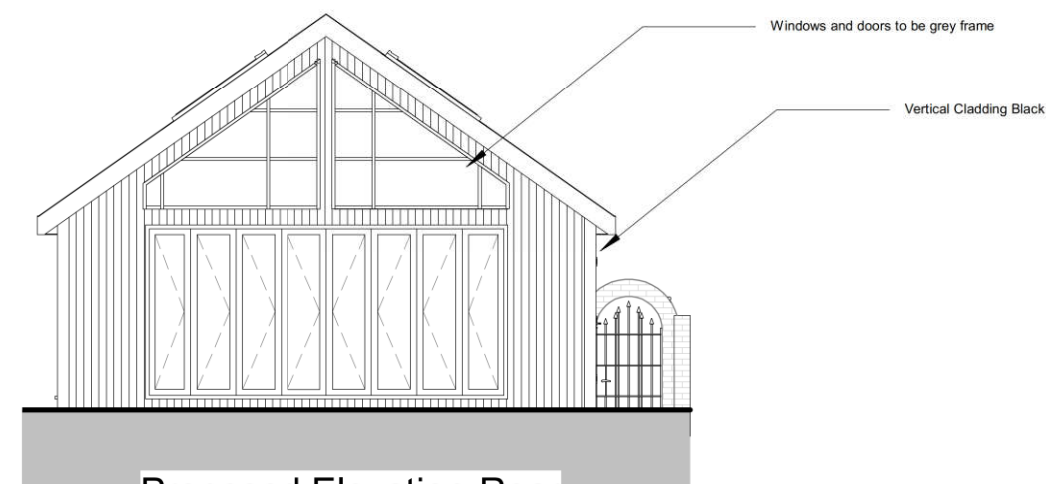
Proposed Elevation-Rear
