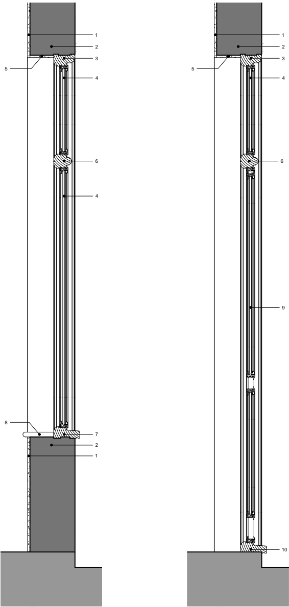
window section 1:20
