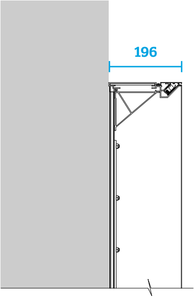
Section Scale 1:10 @ A3
