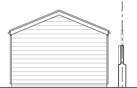
PROPOSED SOUTH ELEVATION - REPLACEMENT ANNEXE SCALE 1:100 @ a3
