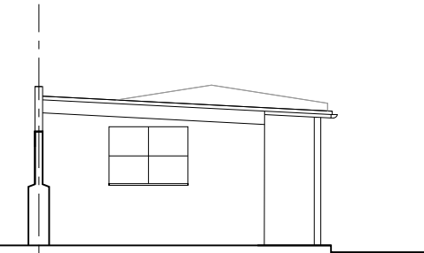
EXISTING NORTH ELEVATION - ANNEXE SCALE 1:100 @ a3
