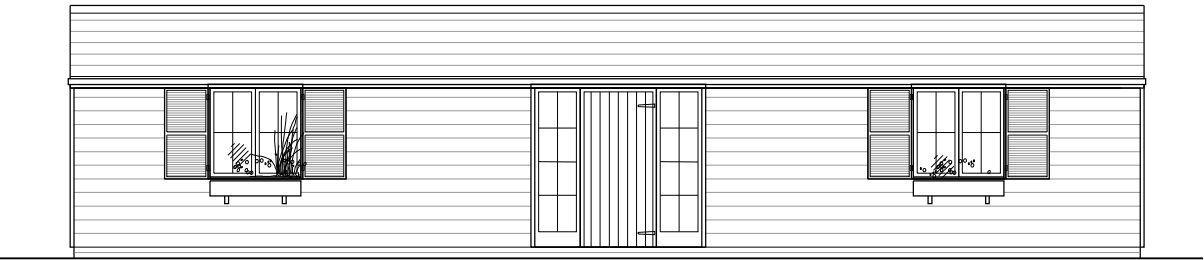
PROPOSED WEST ELEVATION - REPLACEMENT ANNEXE SCALE 1:100 @ a3
