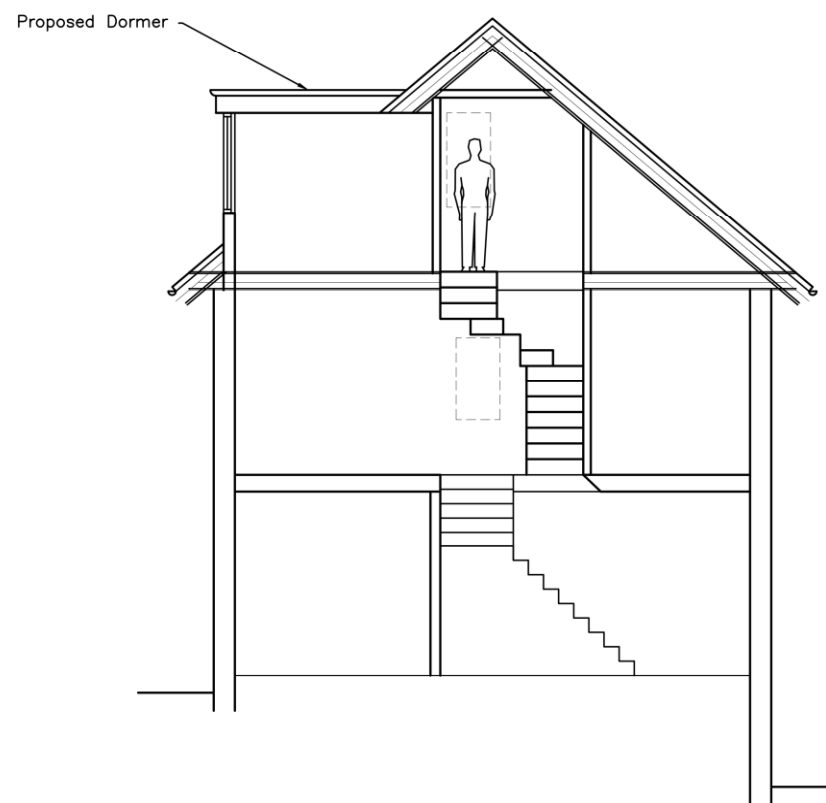
DRAFT SECTION
