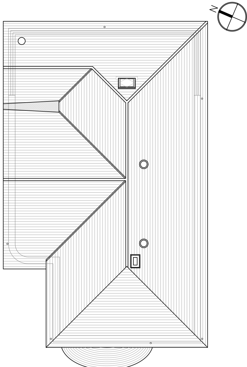
ROOF PLAN 1:100
