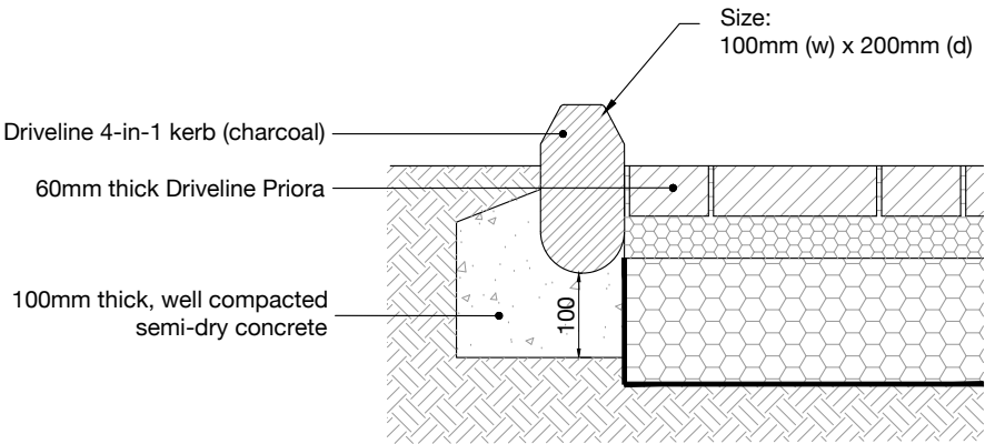
Full Height Kerb
