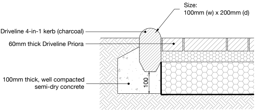
Drop Kerb
