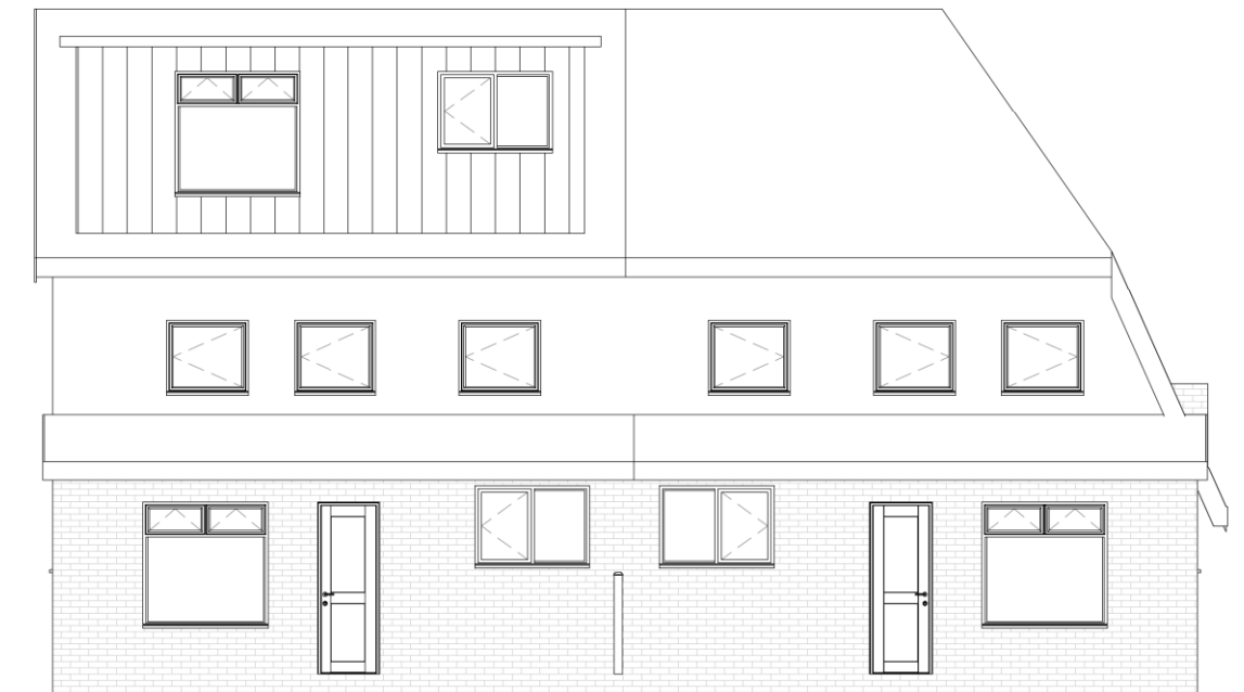
Proposed Elevation-Front
