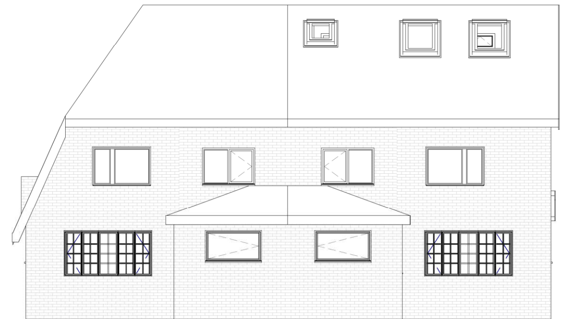
Proposed Elevation-Front
