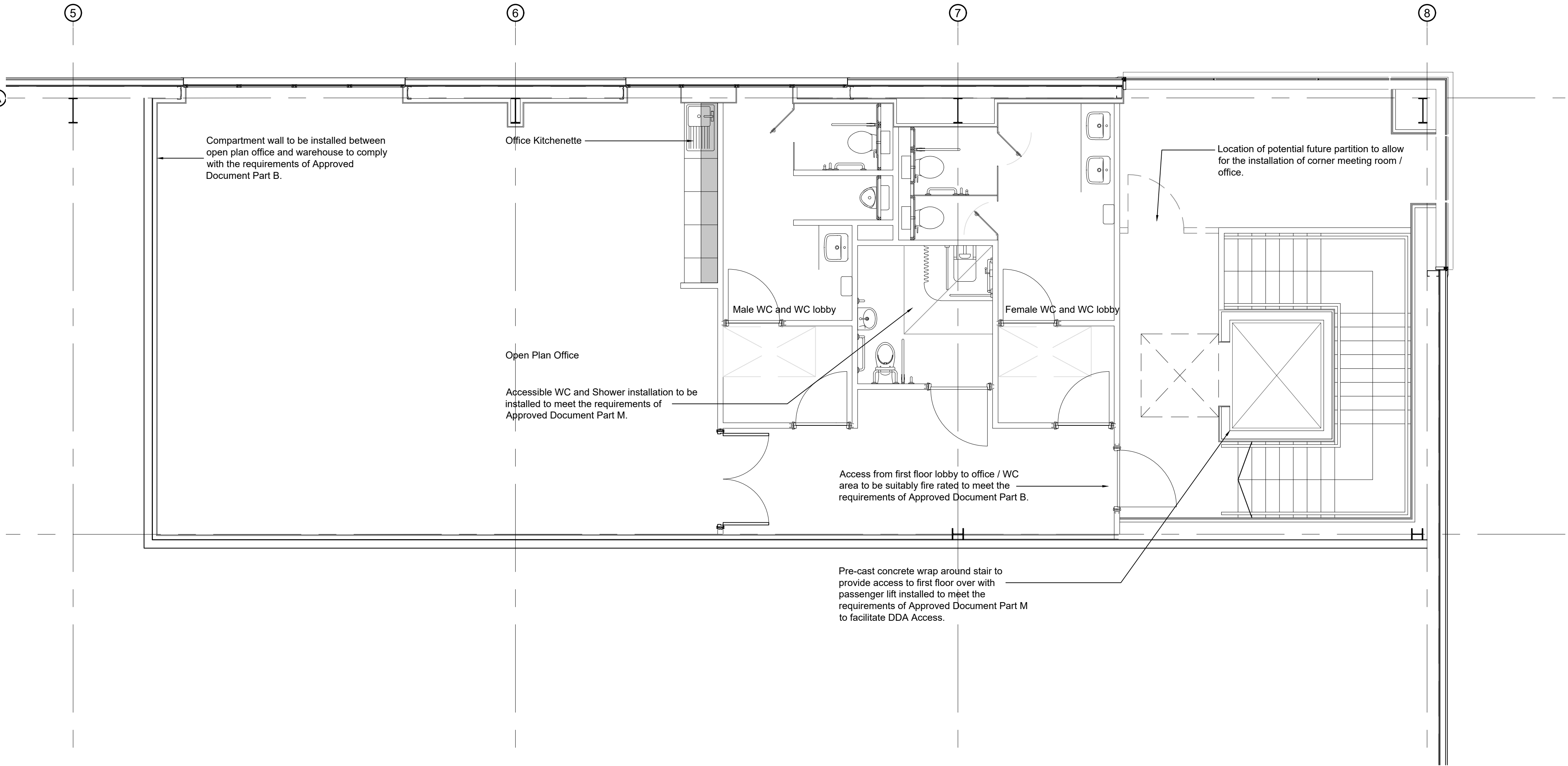
First Floor Office Plan_1:50 @ A1
