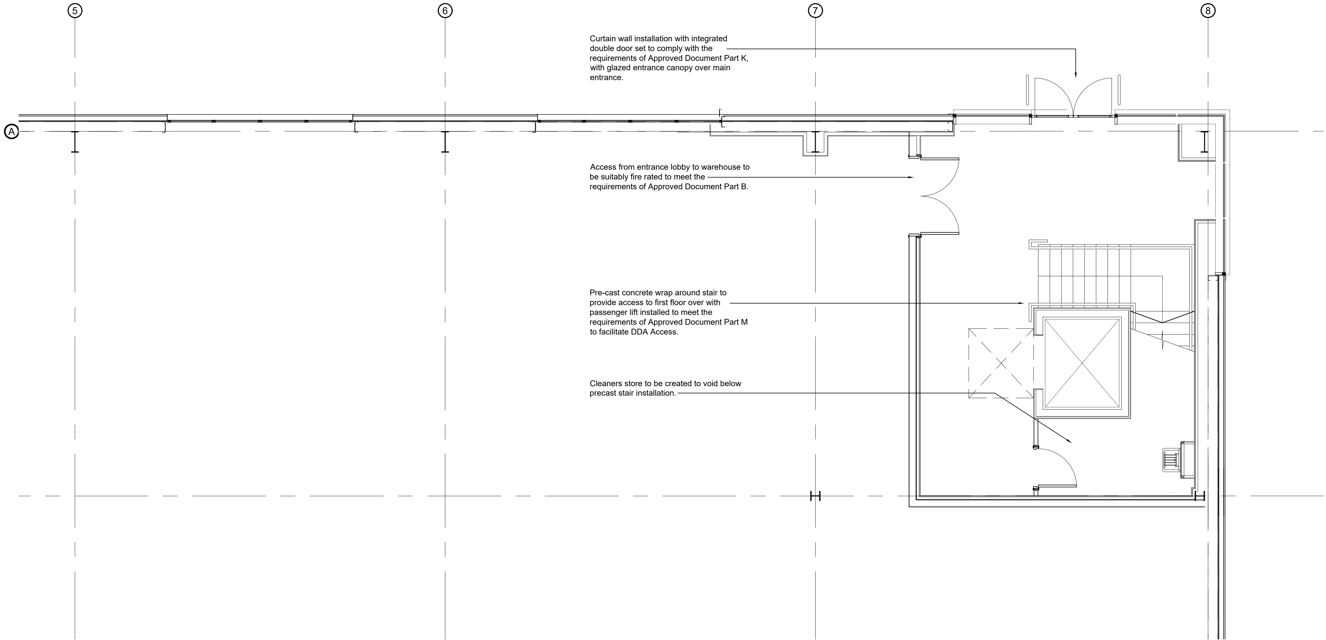
Ground Floor Office Plan_1:50 @ A1
