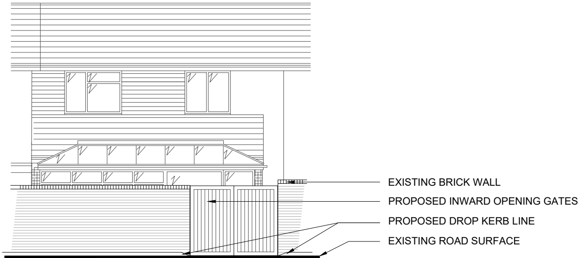
PROPOSED ELEVATION
