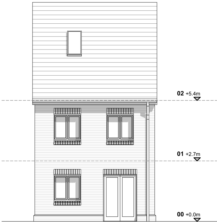
Rear Elevation
