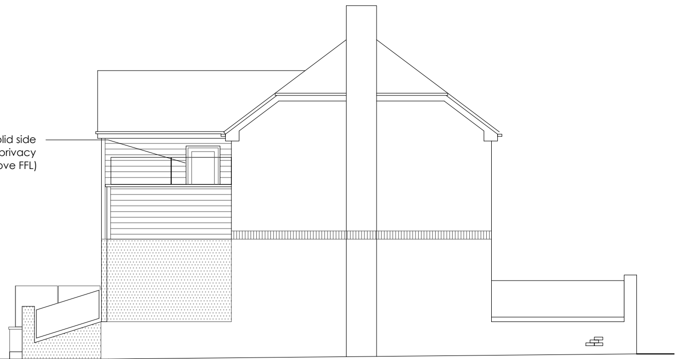
SIDE (E)
