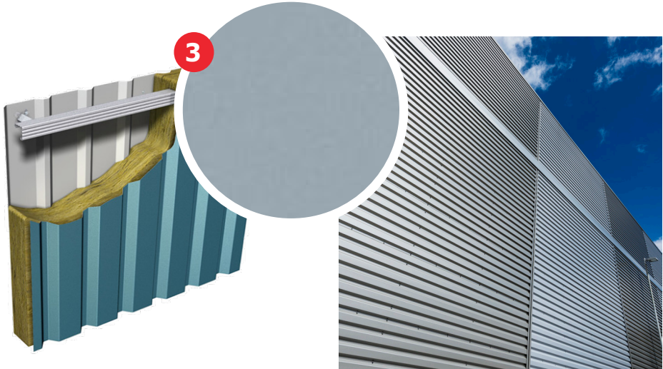
Cladding: Horizontally laid, trapezoidal profile, built up cladding in Colourcoat Prisma Metallic Silver RAL 9006 (3)
