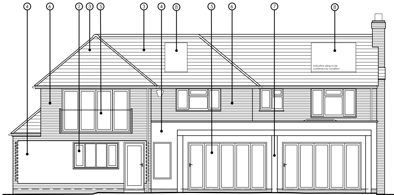
EAST ELEVATION
