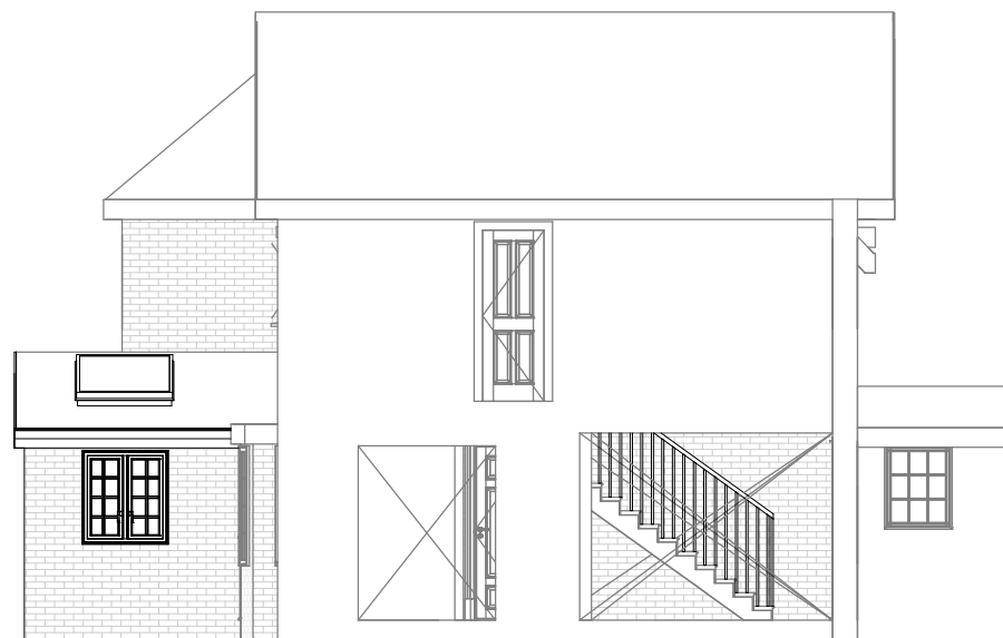
Proposed Side North
