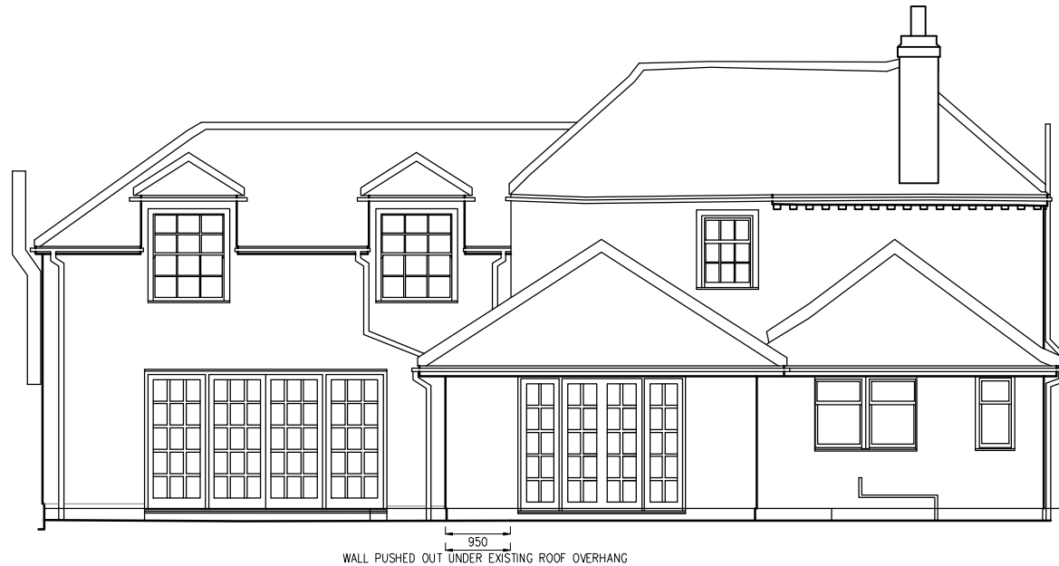
EAST ELEVATION
