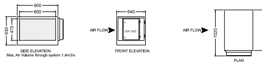
PURIFIED AIR ESP - 3000E PARTICULATE CONTROL UNIT
