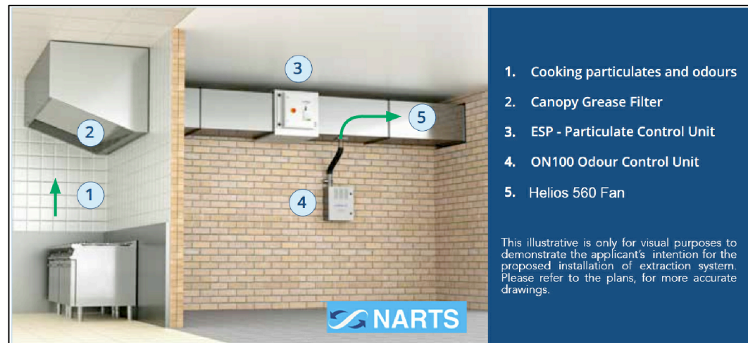
PURIFIED AIR ESP - 3000E PARTICULATE CONTROL UNIT
