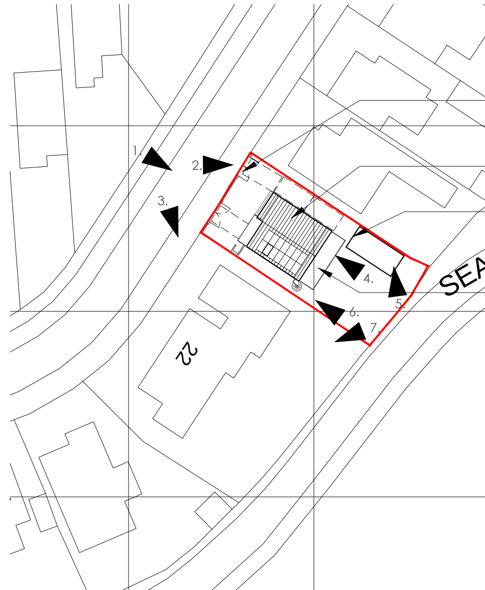
BLOCK PLAN 1:500
