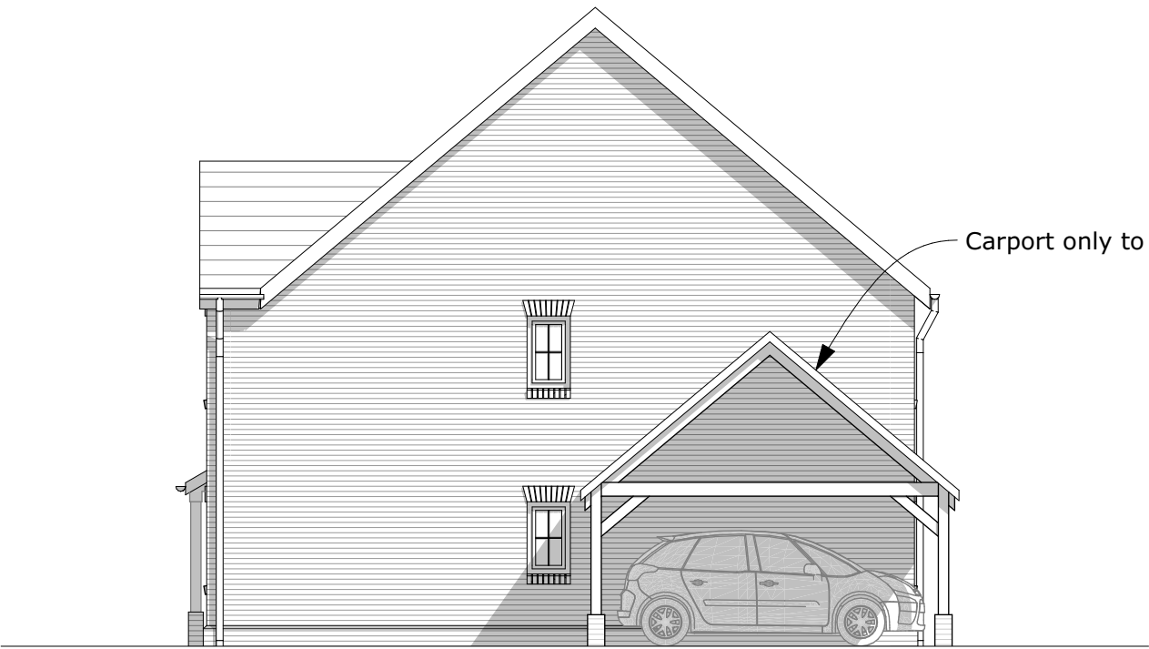
Side 1 Elevation to Plots 33&36
