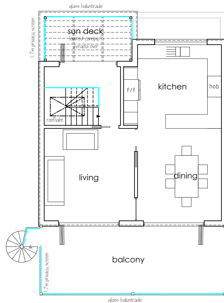
SECOND 1:100
