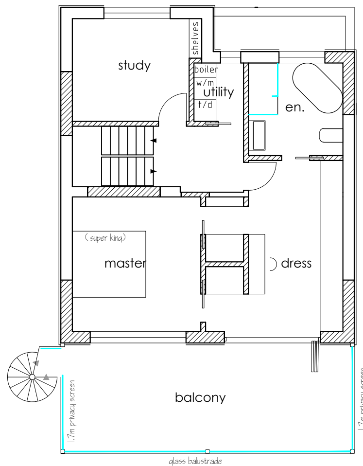
FIRST 1:100
