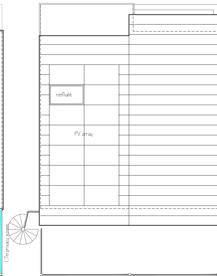
ROOF 1:100
