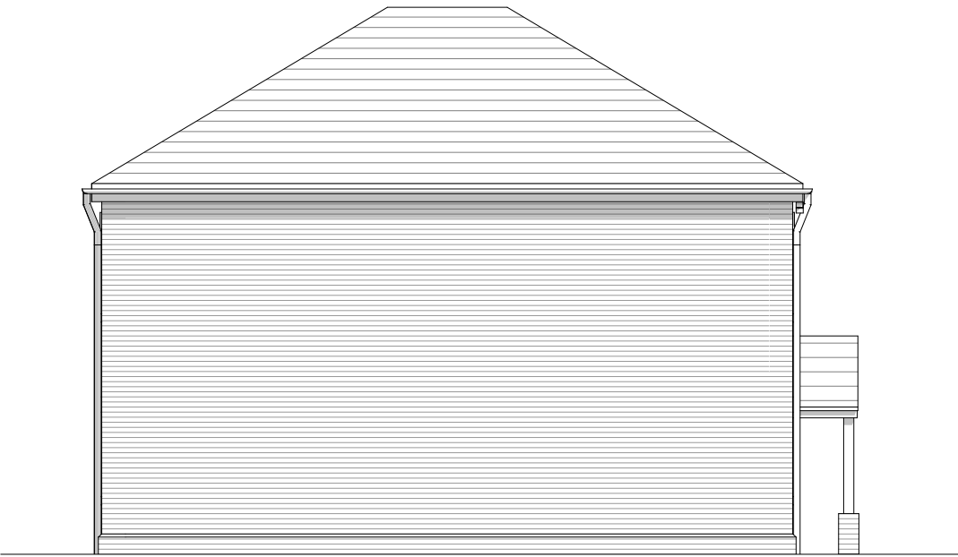
Side 1 Elevation
