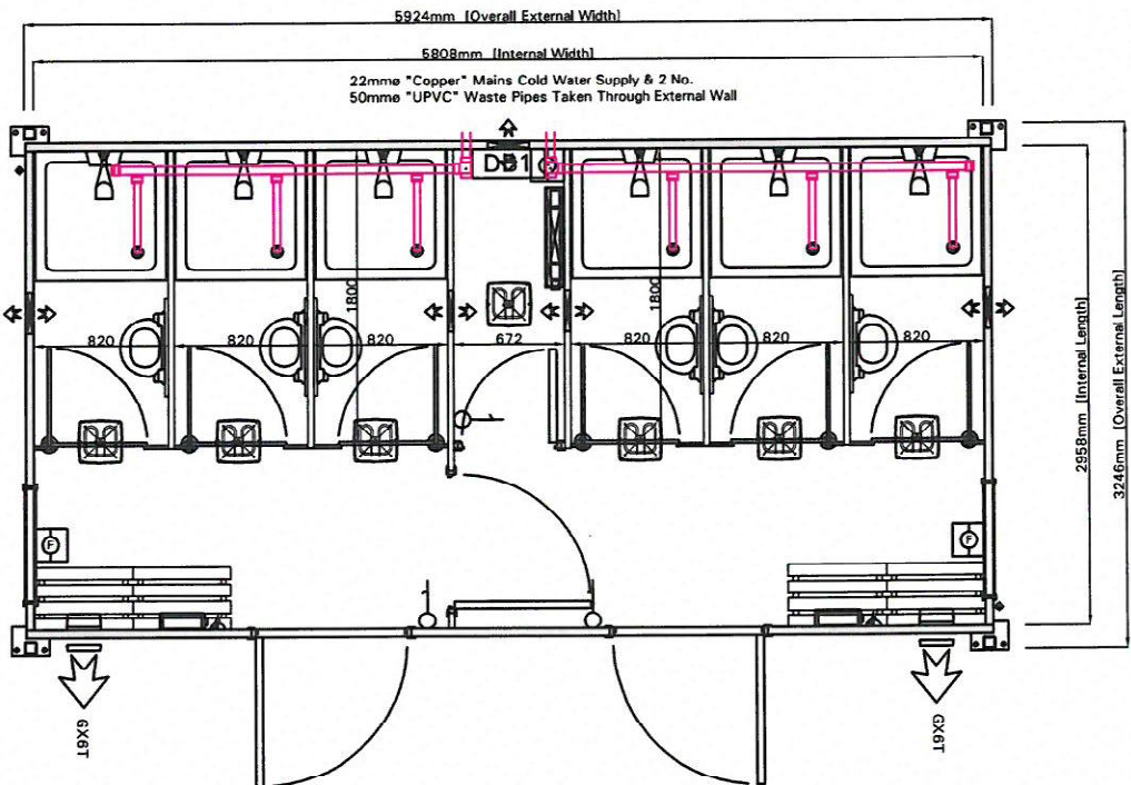
Floor Plan [Standard]
